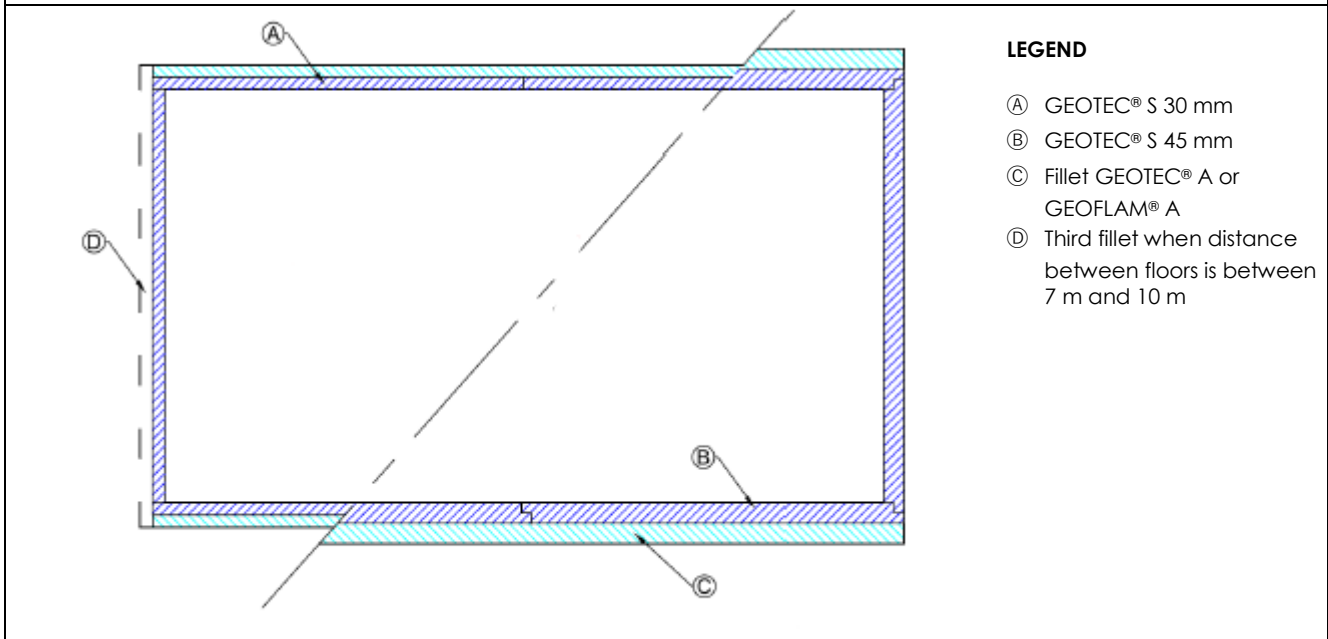
Figure 2.2.4.4.1c: Vertical duct composed of 6 or more boards, with 1 board on the short side
