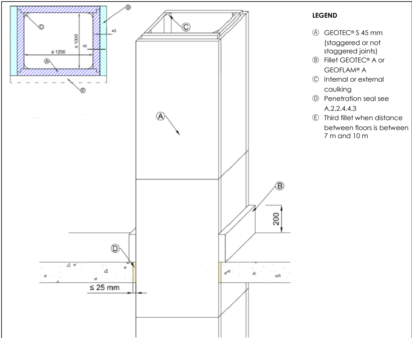
Figure 2.2.4.4.1b: Vertical duct composed of 45 mm GEOTEC® S fire protective boards
